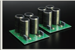
Cumulative 80,000µF filtering capacitors
