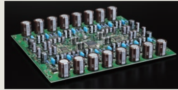
D/A converter driving 8 parallel channels
